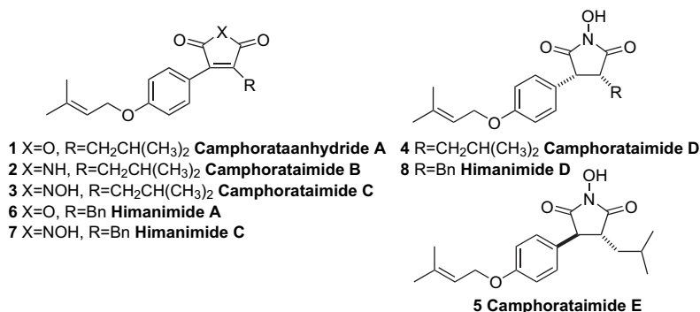
Figure 1. Maleic anhydride and maleimide natural products of Antrodia camphorate and himanimide.
